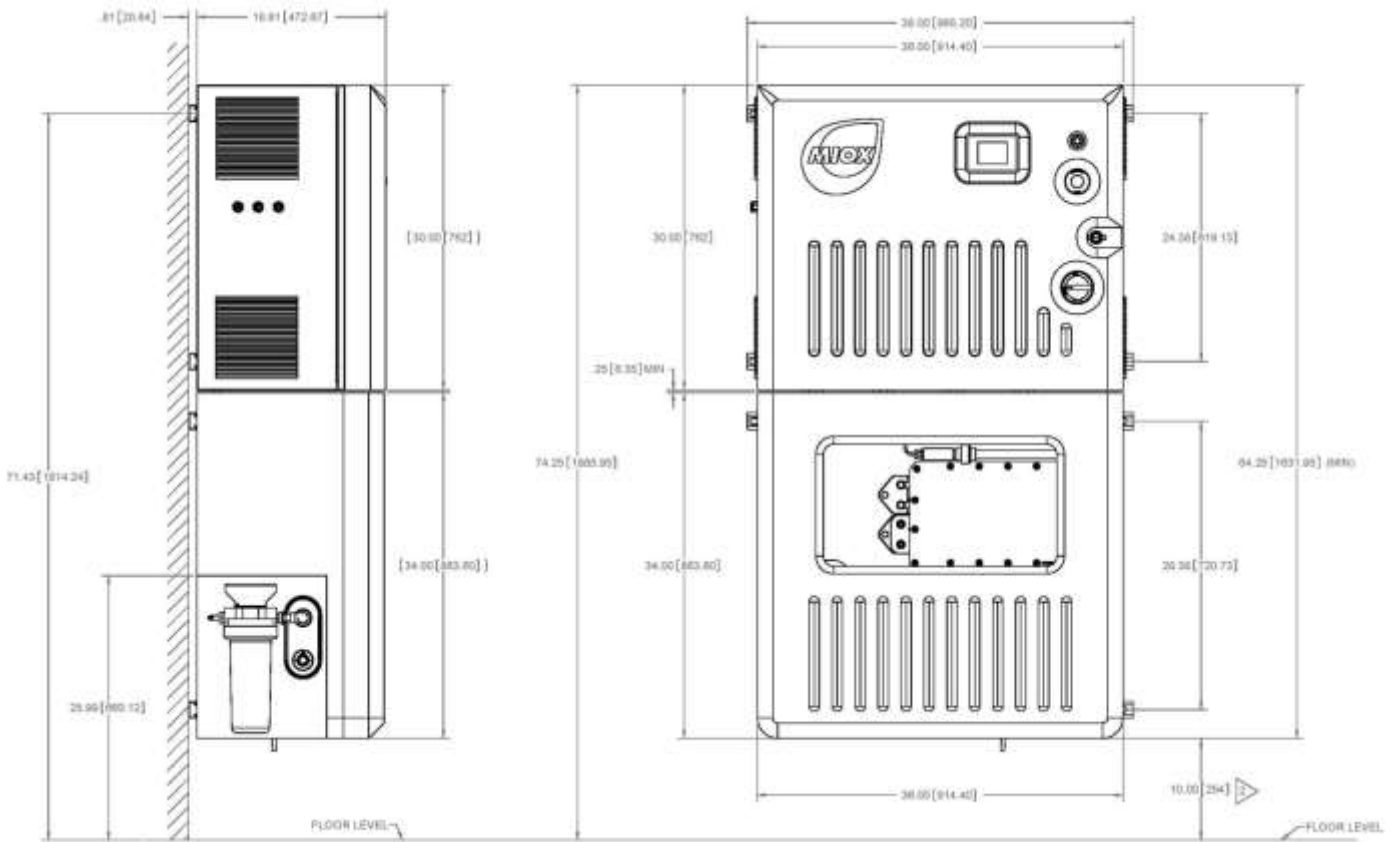
Vault™ Self Cleaning MIXED OXIDANT Drawing
